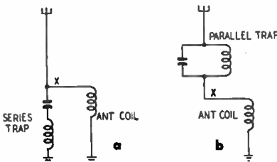
Fig. 7—Tuned circuits employed as wavetraps.
