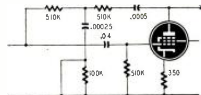
Removing short from resistor decreases highs.
