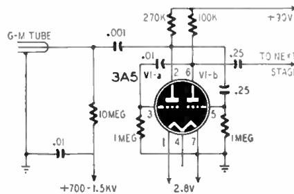
Fig. 3—Tube is quenched by a negative pulse.
