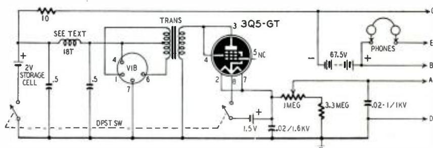
Fig. 1—This is the schematic diagram of the power-supply components inside the main case.
