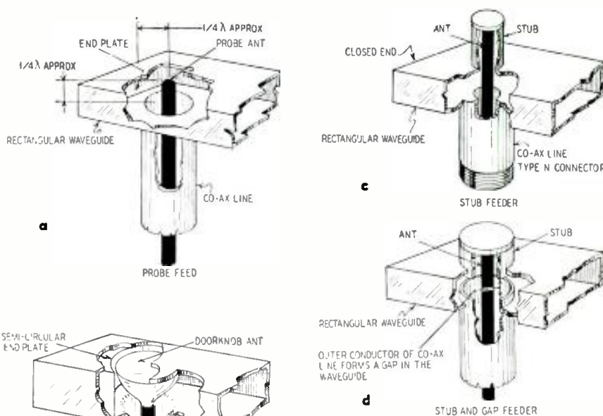
Fig. 4—Four waveguide-to-co-axial sections.
