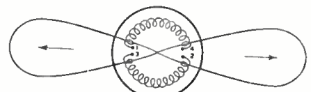
Fig. 4—Inductive Transpole field pattern.
