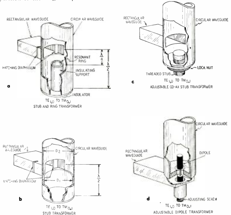
Fig. 3.—These are waveguide transformers used to match circular guides to rectangular ones.
