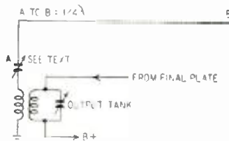
Fig. 4—Marconi antenna was prewar favorite.
