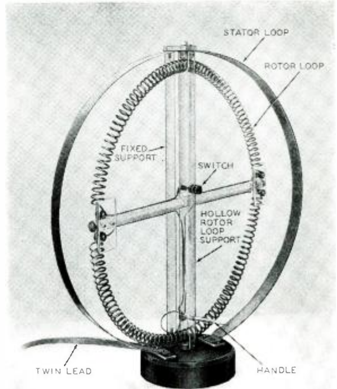
The Inductive Transpole Variotenna introduces some new principles.
